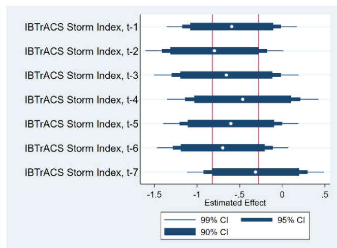
Fig. 5. Lagged Effects of Storms on Democracy Notes: These figures depict the coefficients associated with the regression model reported in columns (7) and (8) of Appendices A14 and A15, respectively.
