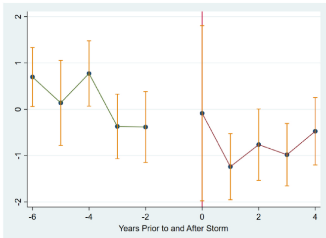
Fig. 4. Event Study Estimates of the Effect of Storms on the Polity Measure of Democracy
